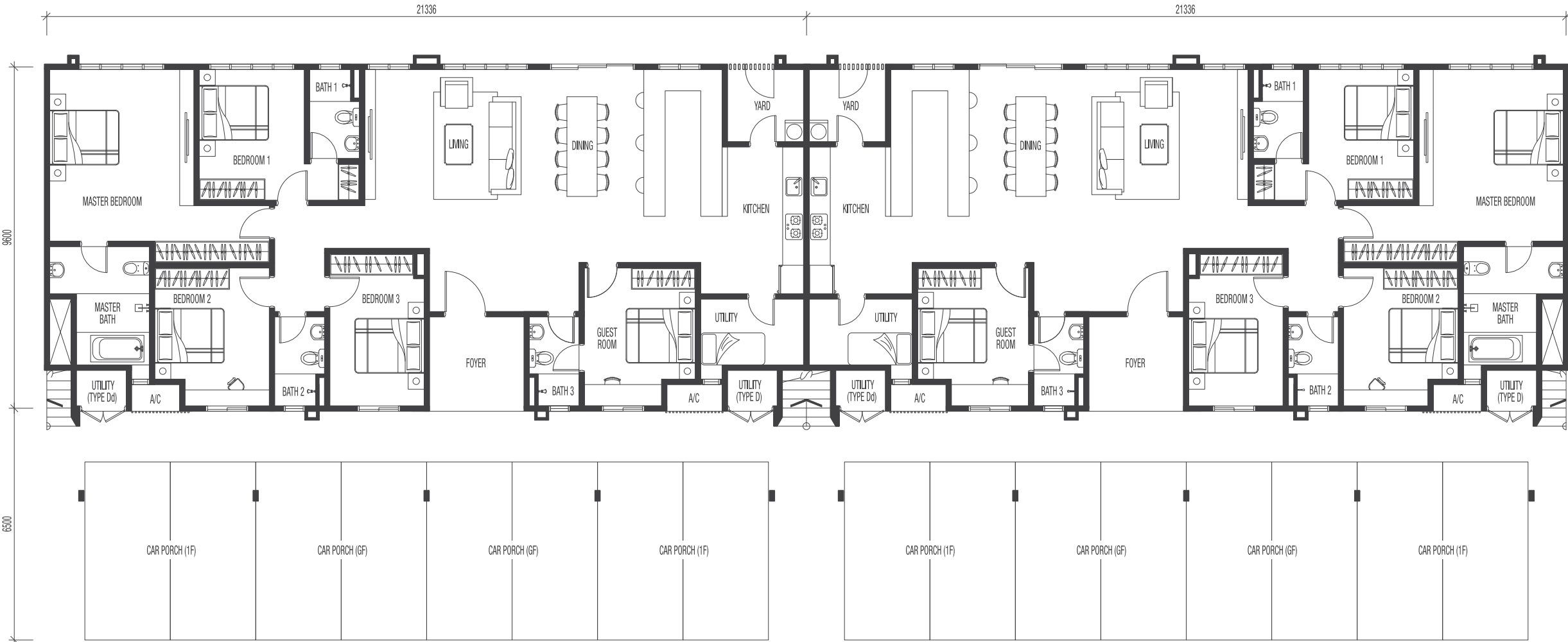
GROUND FLOOR
